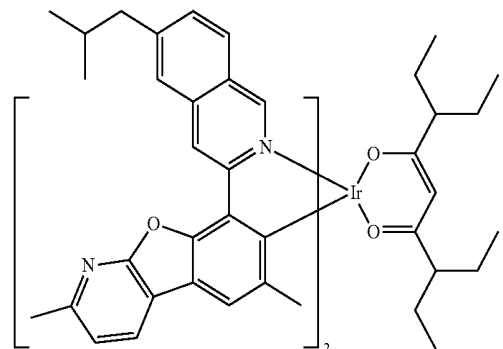
Compound 32
