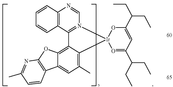
Compound 52
