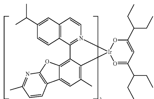
Compound 44
