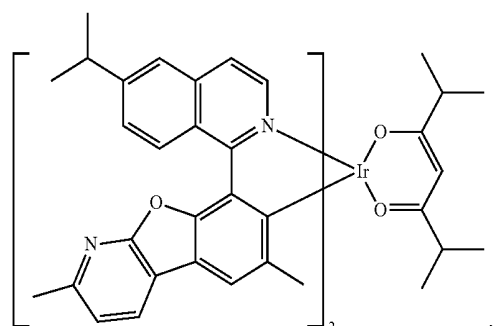
Compound 45
