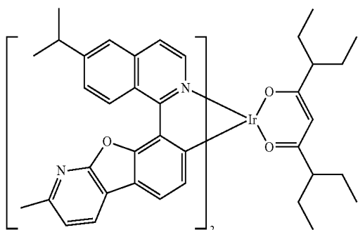
Compound 43
