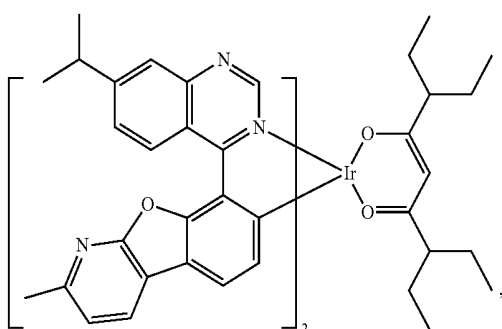
Compound 54
