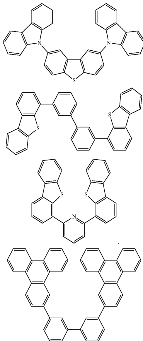
Compound 59
