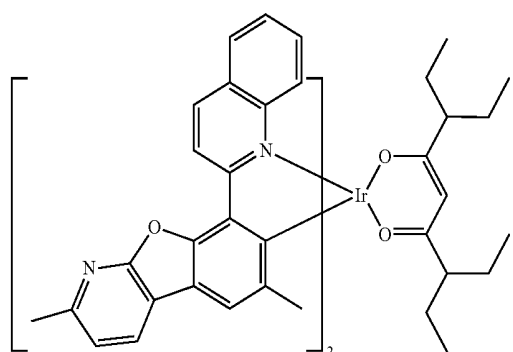
Compound 20
