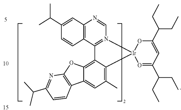
Compound 60
