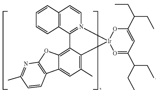
Compound 40
